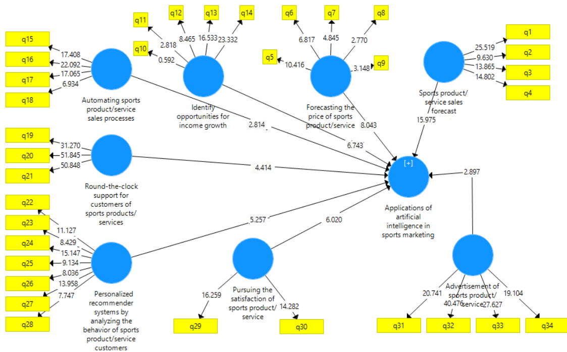
Figure 2. The Final Structural Model of The Research with Critical Values (T-Statistics)
